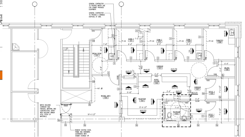
01 FLOOR PLAN SCALE: 1/4" = 1'-0"
