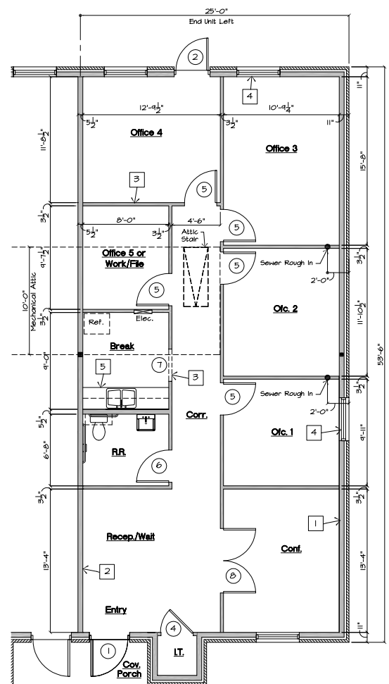
Office Floor Plan - End Unit Right 1,358 SF Building Types I & II Scale: 1/4" = 1'-0"
