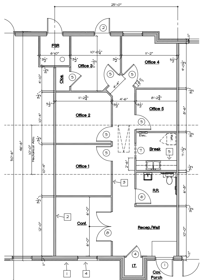
Office Floor Plan - Center Unit Right 1,167 SF Building Type III Scale: 1/4" = 1'-0"
