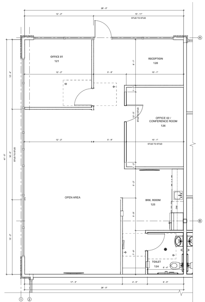
A2 DIMENSIONED FLOOR PLAN A-111 5/21/17
