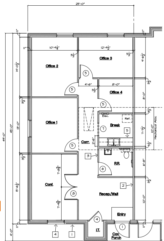
Office Floor Plan - End Unit Left 1,145 SF Building Type III Scale: 1/4" = 1'-0"
